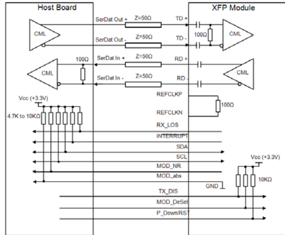
Figure3. Recommended High-speed Interface Circuit
