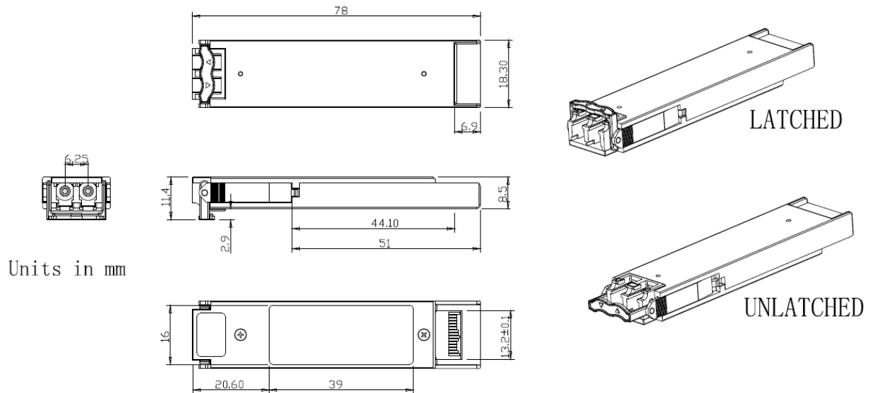
Figure5. Mechanical Specifications
