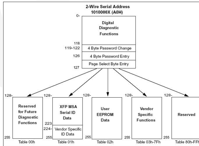
Figure4. 2-wire Serial Digital Diagnostic Memory Map
