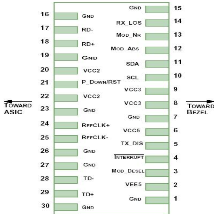
Figure1.Electrical Pin-out Details
