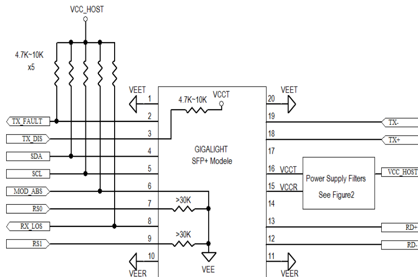
Figure2. Host-Module Interface
