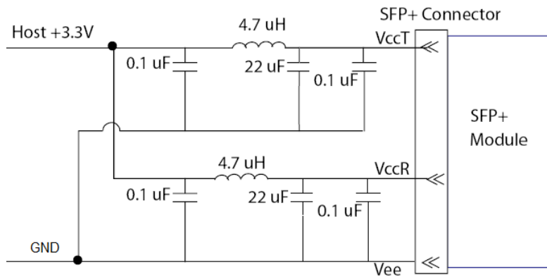
Figure1. Host Board Power Supply Filters Circuit
