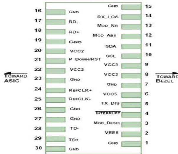
Figure1.Electrical Pin-out Details
