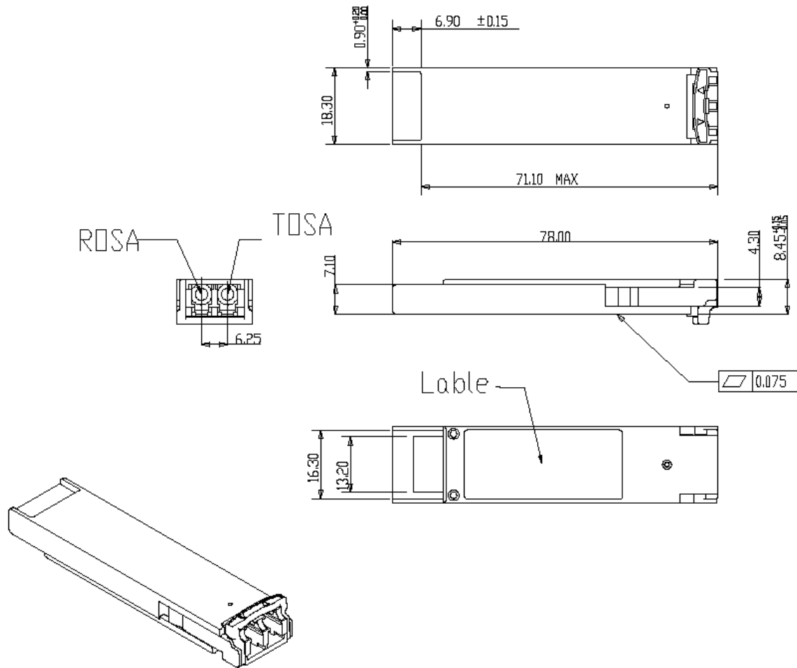
Figure6. Mechanical Specifications
