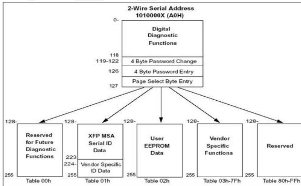
Figure 1.2-wire Serial Digital Diagnostic Memory Map
