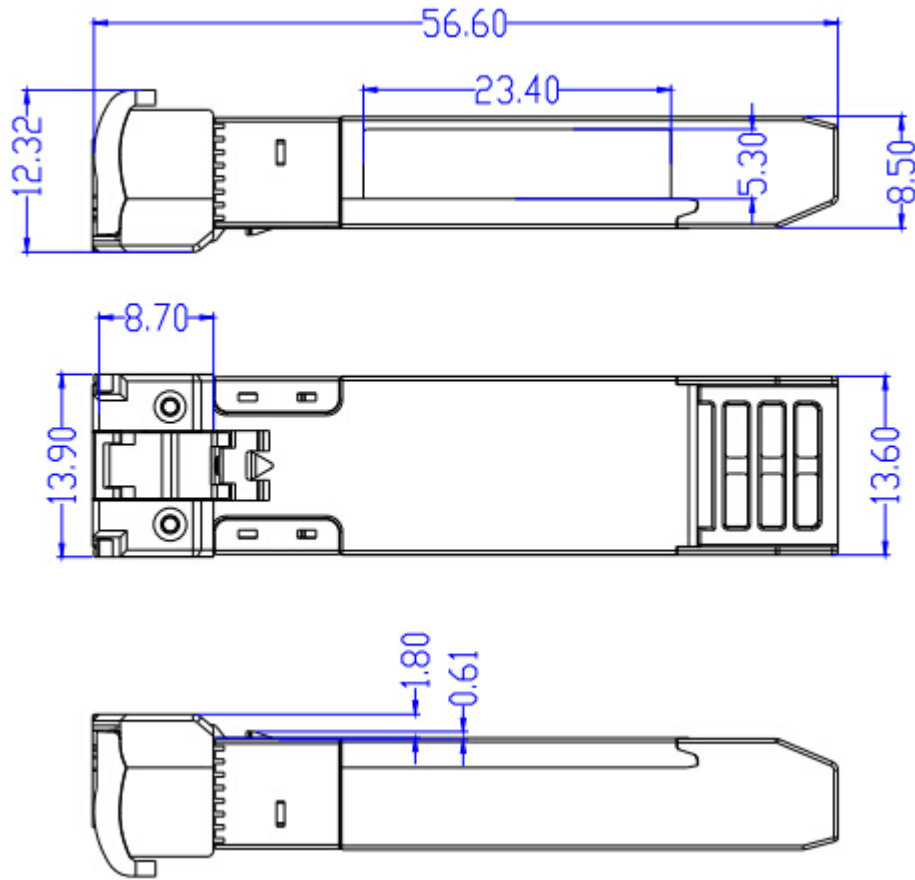
Figure4. Mechanical Specifications
