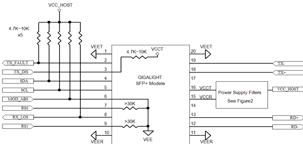
Figure3. Host-Module Interface
