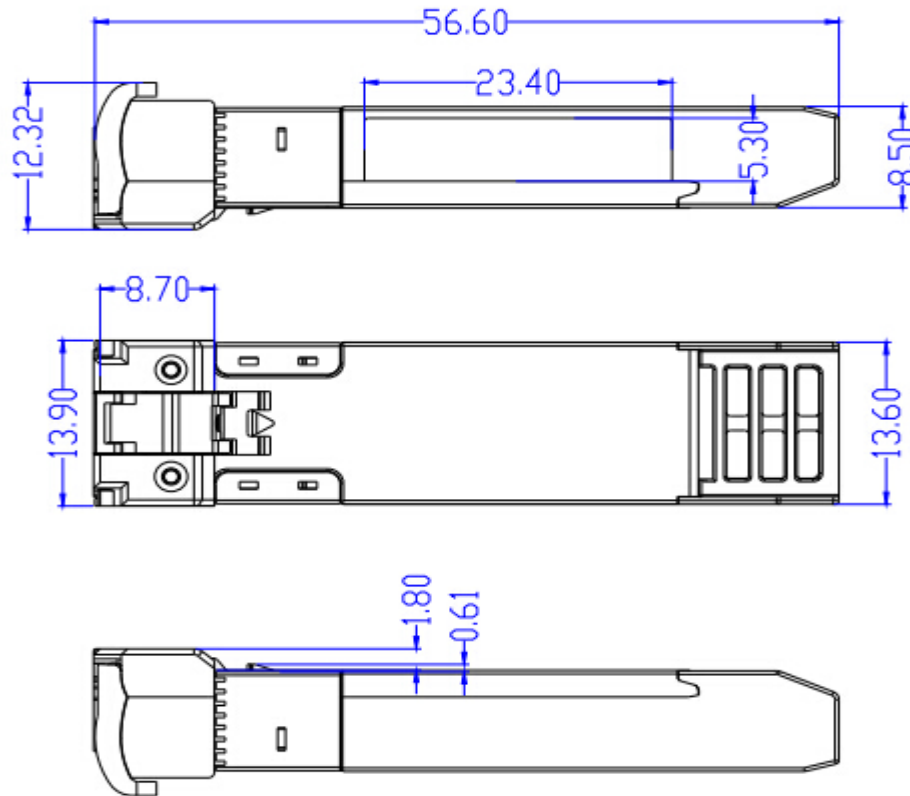
Figure6. Mechanical Specification
