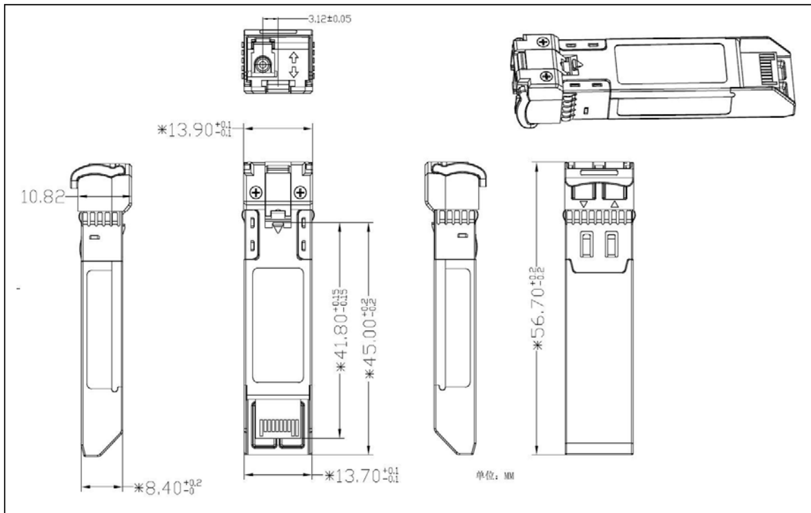
Package Dimensions
