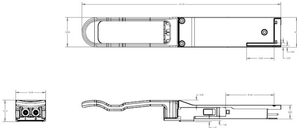
Figure 2 –mechanical drawing
