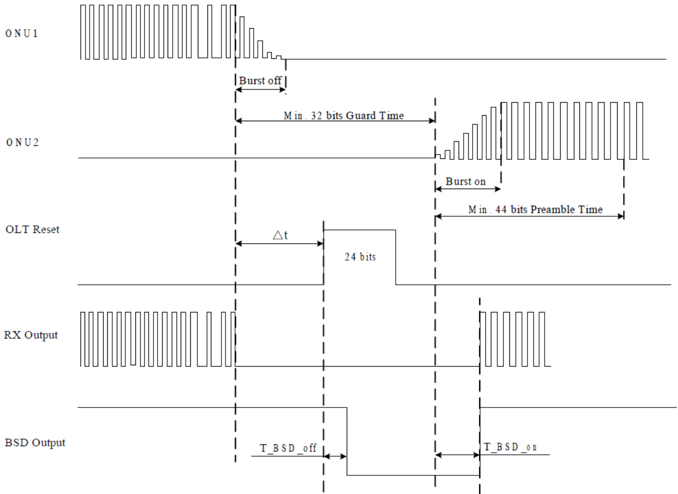
Figure 2 Reset Timin
