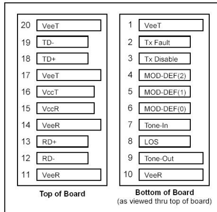
Figure1.Electrical Pin-out Details
