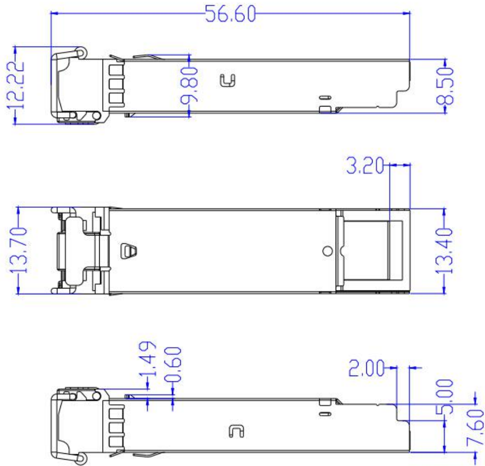
Figure5. Mechanical Dimensions
