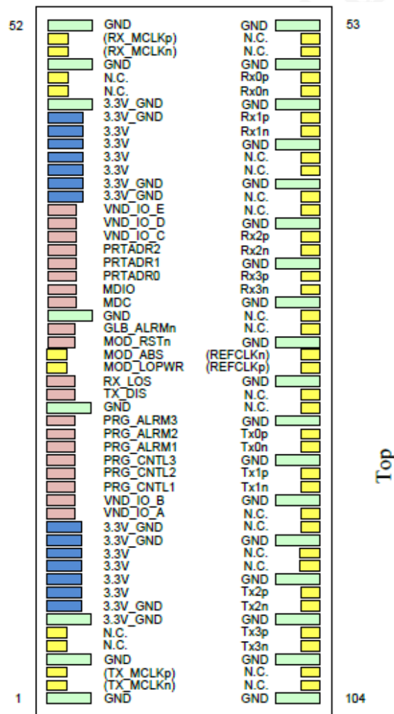
Figure 2 CFP2 optical transceiver pin-out
